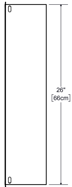
Side View(Right)
