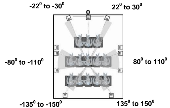
Figure 3 – A simple diagram showing the angular ranges within which loudspeakers should be located relative to the prime listening location for a 7.1 system. From CEA/CEDIA-CEB22
