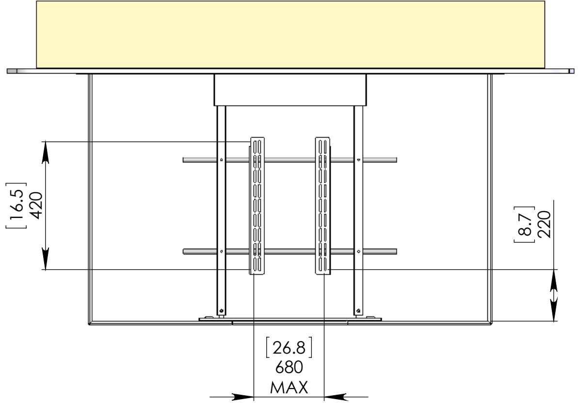
Front View on Screen Mount
