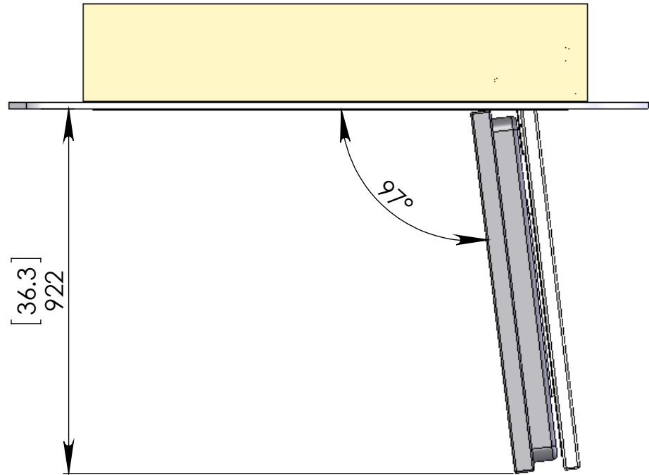
Side View at Max Tilt
