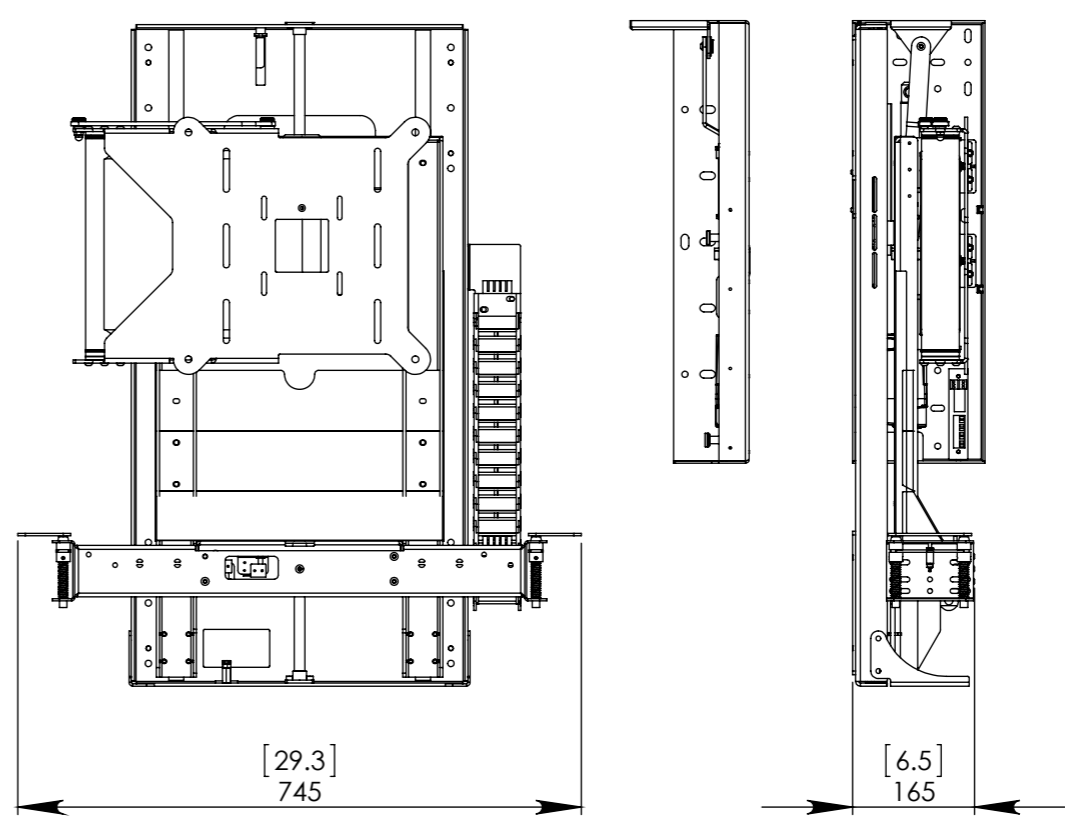
MECHANISM - DOWN POSITION
