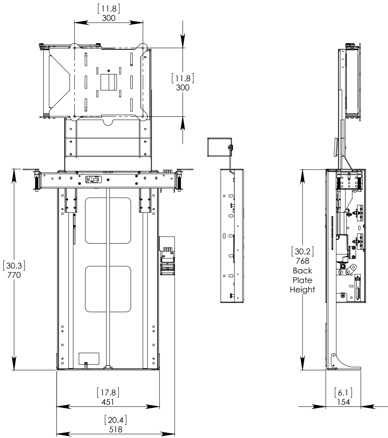
MECHANISM - UP POSITION
