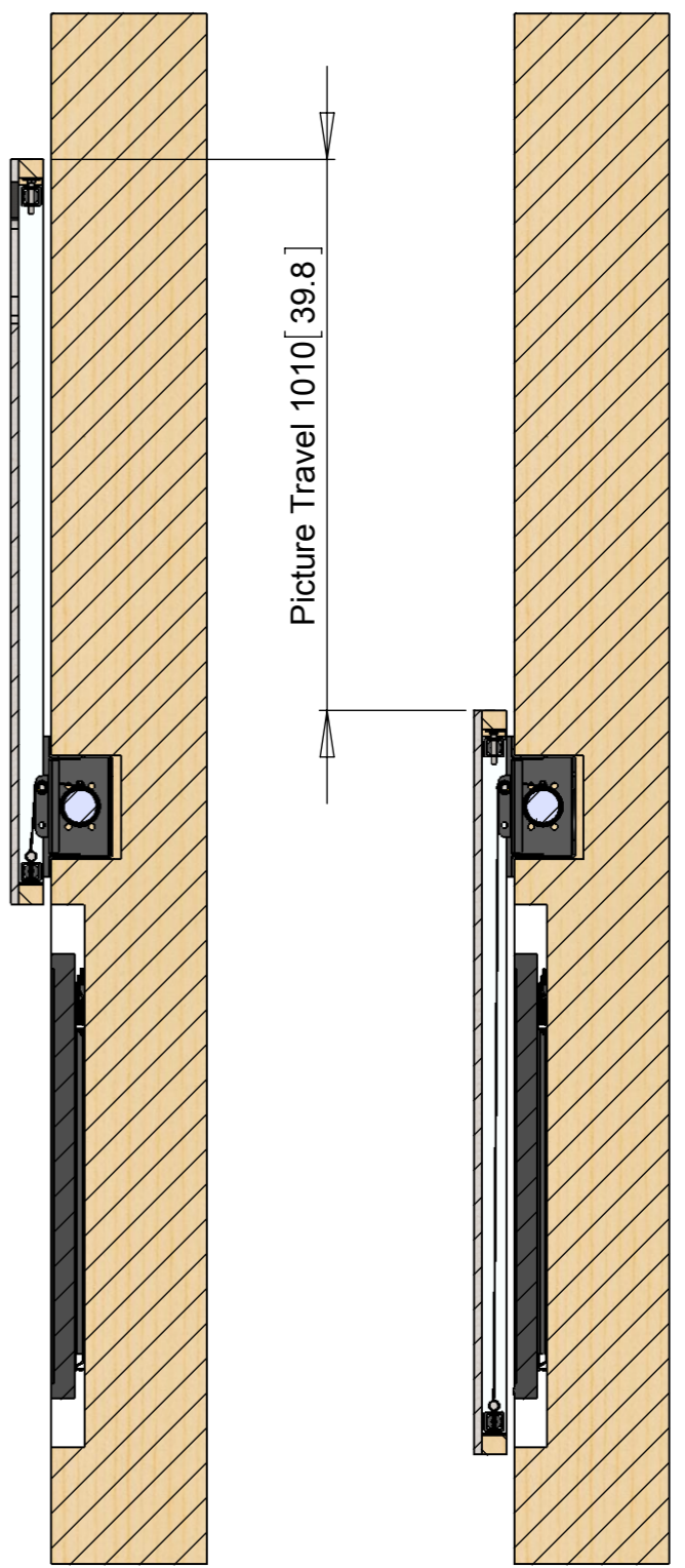
UP POSITION
